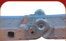
SAFETY LOCK CUM HINGES
